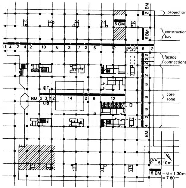
1 Basle Cantonal Hospital: schematic ground floor plan
